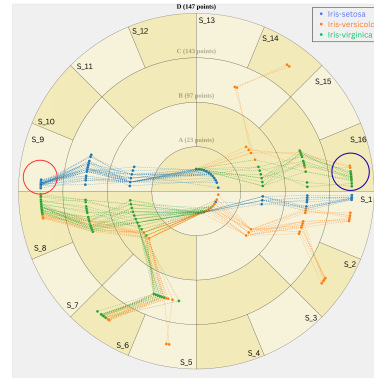
(b) RAYS Visualization for Feature Set 2
