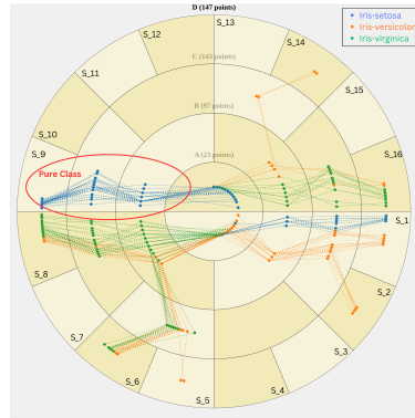
(a) RAYS Visualization for Feature Set 1
